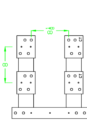
K4797 MOUNTING STUDS 1Ø3W OR 3Ø3W
